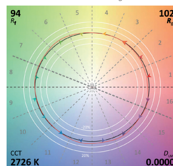
Colour vector diagram
